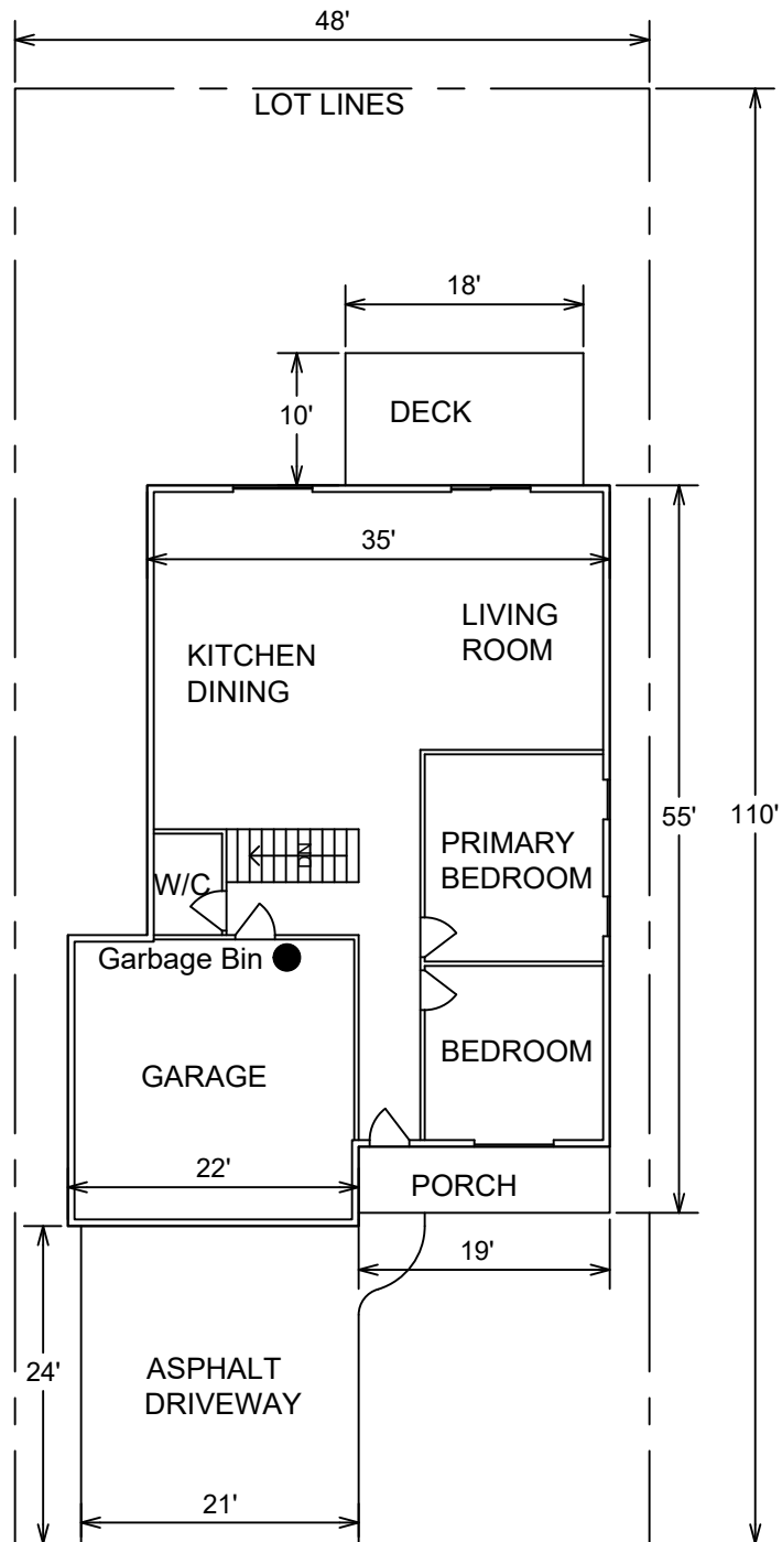
SITE PLAN
